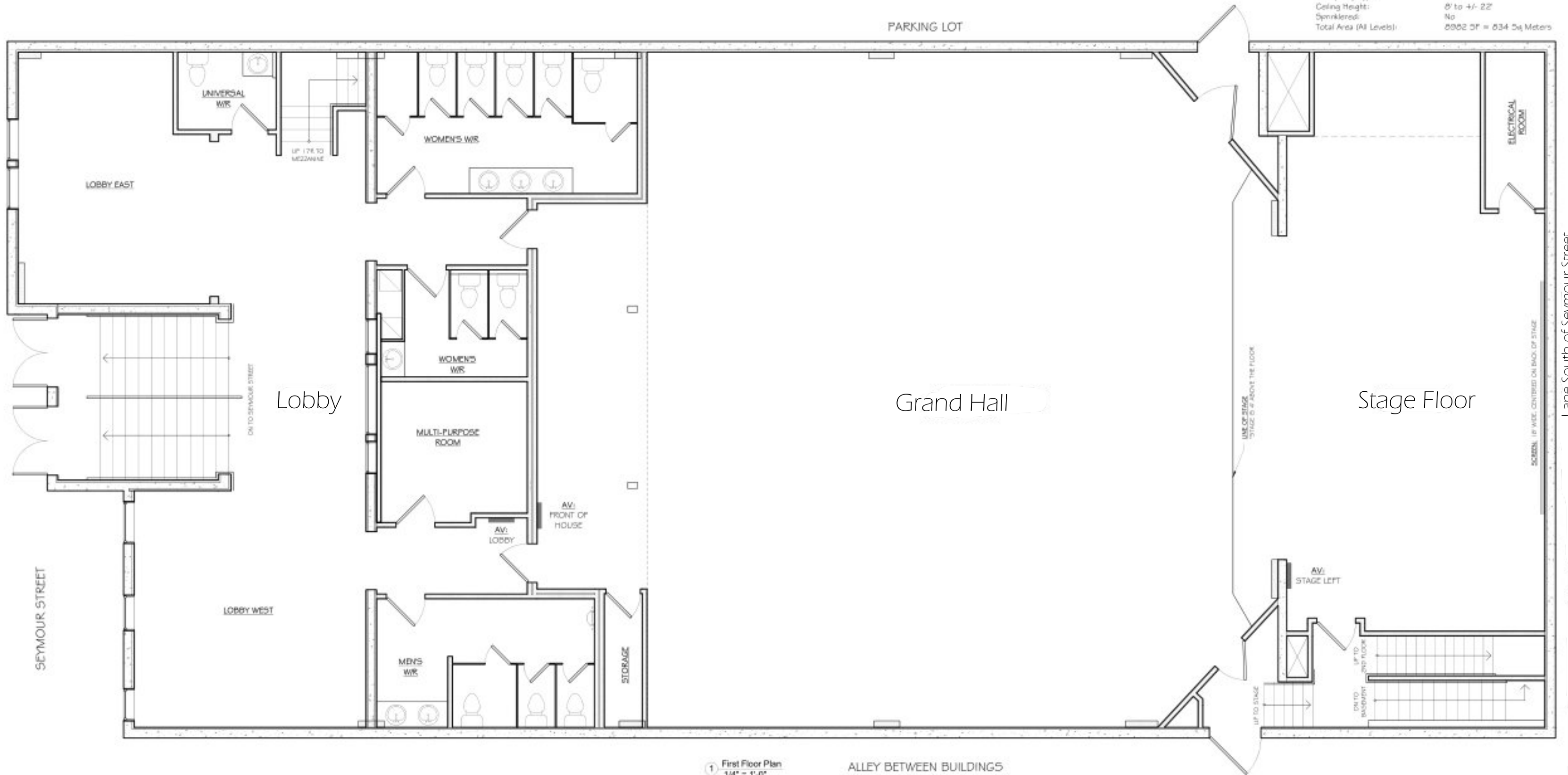
1 First Floor Plan 1/4" = 1'-0"
